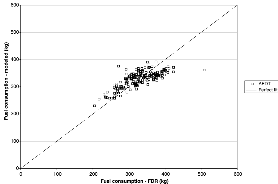
Fig. 3 Comparison of FDR and AEDT-modeled fuel consumption for Boeing 757-200 departures to 3000 ft AFE.
