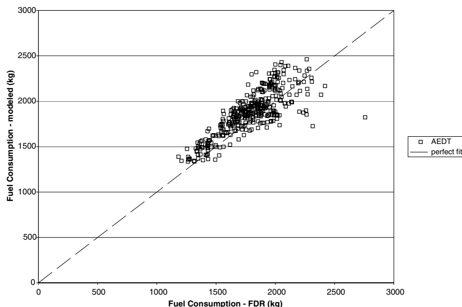
Fig. 4 Comparison of FDR and AEDT-modeled fuel consumption for Boeing 777-300ER departures to 10,000 ft AFE.
