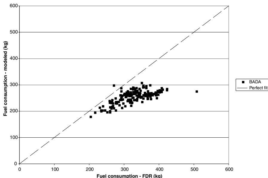
Fig. 1 Comparison of FDR and BADA-modeled fuel consumption for Boeing 757-200 departures to 3000 ft AFE.
