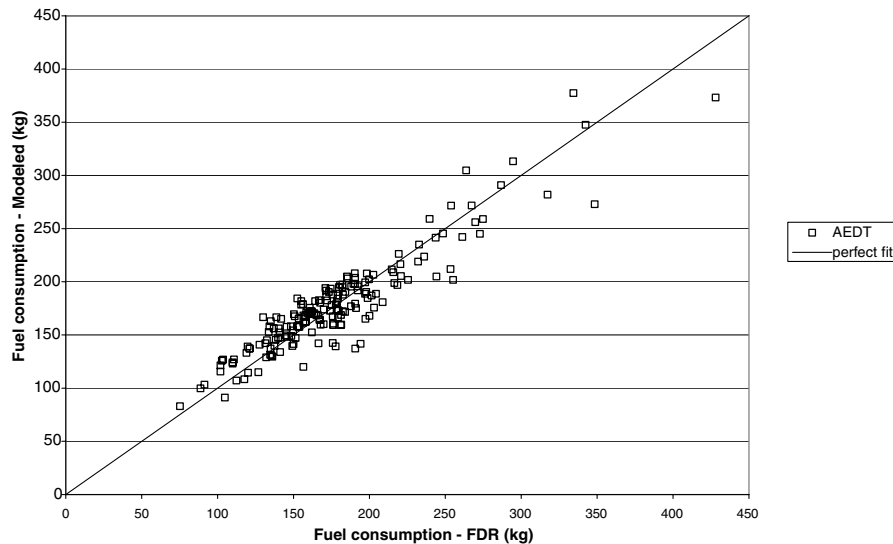
Fig. 5 Comparison of FDR and AEDT-modeled fuel consumption for Boeing 757-200 arrivals from 3000 ft AFE.
