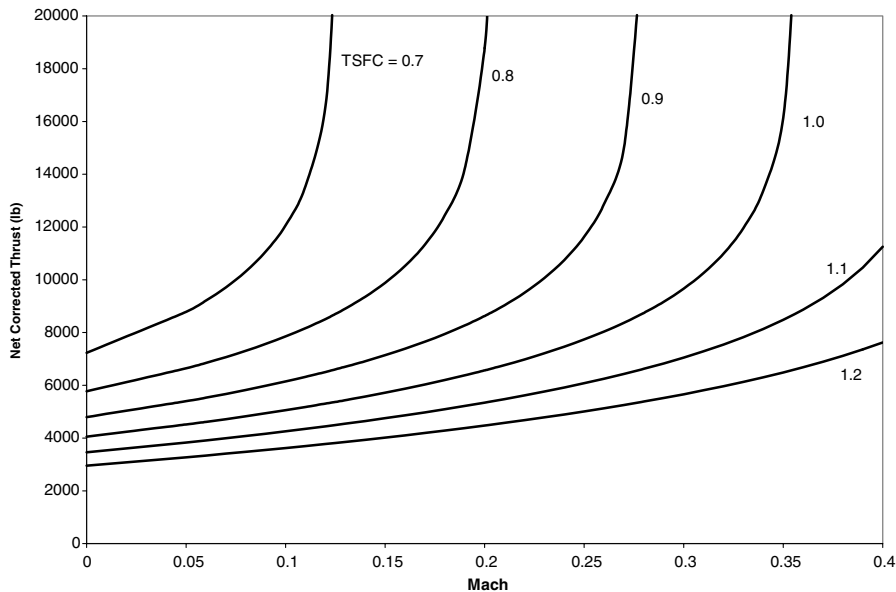
Fig. 2 Example arrival TSFC curves generated with Eq. (2).
